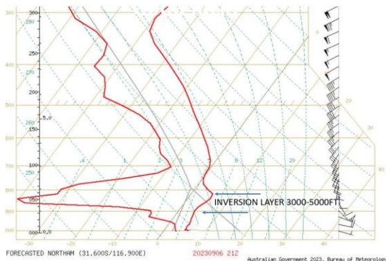
FORECASTED NORTHM (31.600S/116.900E) 20230906 21Z Australian Government 2023, Bureau of Meteorology
