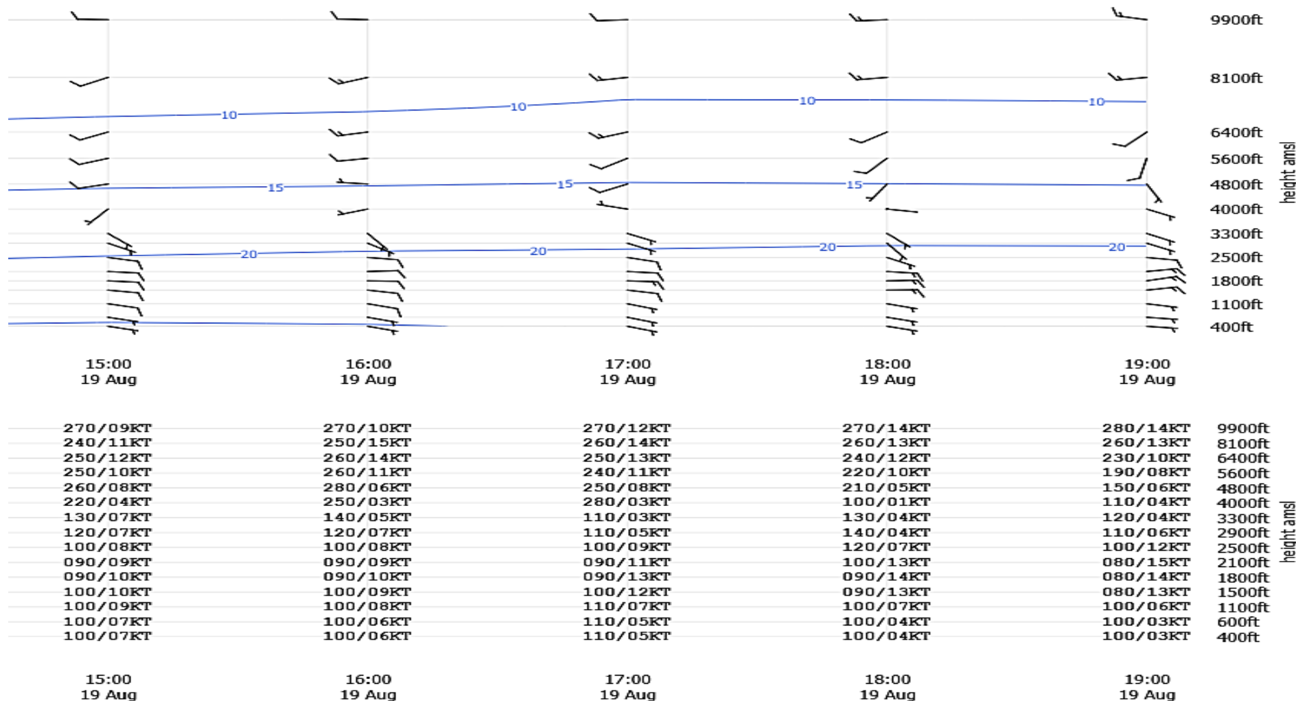
FCST Model Arome in UTC, dd from, ff [kt]
